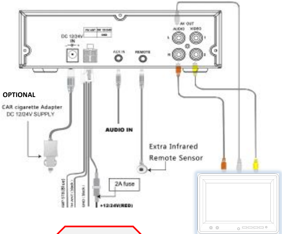
UNIVERSAL LCD MONITOR
